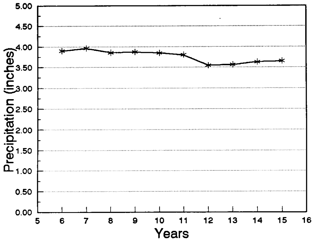
Figure A.5 Sensitivity analysis for precipitation volume given a 72 hour Inter-Event Dry Period and a 3 month Return Period for Inglis as a function of the number of years of data.
