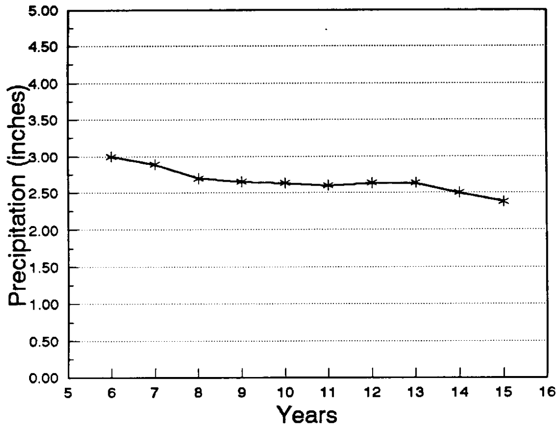
Figure A.7 Sensitivity analysis for precipitation volume given a 72 hour Inter-Event Dry Period and a 3 month Return Period for Key West as a function of the number of years of data.
