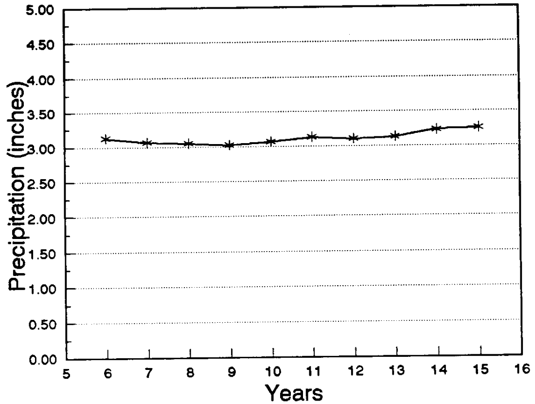
Figure A.6 Sensitivity analysis for precipitation volume given a 72 hour Inter-Event Dry Period and a 3 month Return Period for Jacksonville as a function of the number of years of data.
