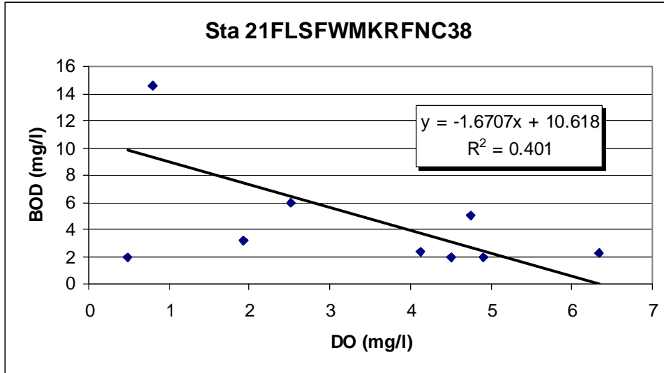
Figure E-1. Correlation between DO and BOD in WBID 3186B
