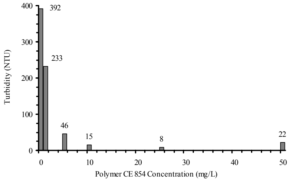
Figure 2. The relationship between dosage concentration and turbidity for Hyperfloc CE 854, a polyacrylamide copolymer with a high degree of cationic charge and with a very high molecular weight.
