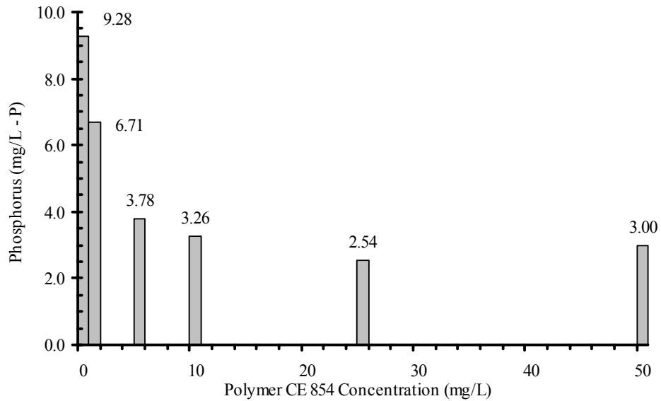
Figure 3. The relationship between dosage concentration and Soluble Reactive Phosphorus for Hyperfloc CE 854, a polyacrylamide copolymer with a high degree of cationic charge and with a very high molecular weight.
