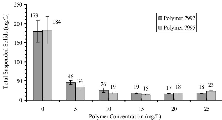
Figure 4. Total Suspended Solids removed using very high degree of cationic charge, high molecular weight polymer.
