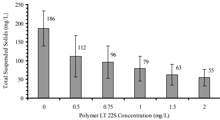
Figure 5. Total suspended solids removed using low degree of anionic charge, high molecular weight polymer.
