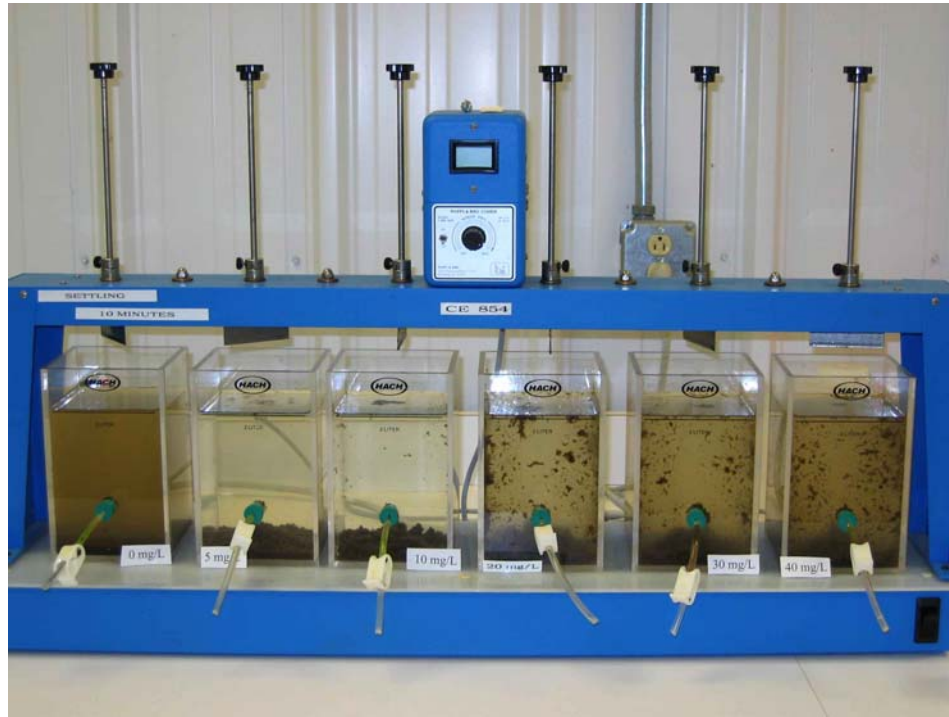
Figure 1. Phipps & Bird Six-paddle stirrer with illuminated base.
