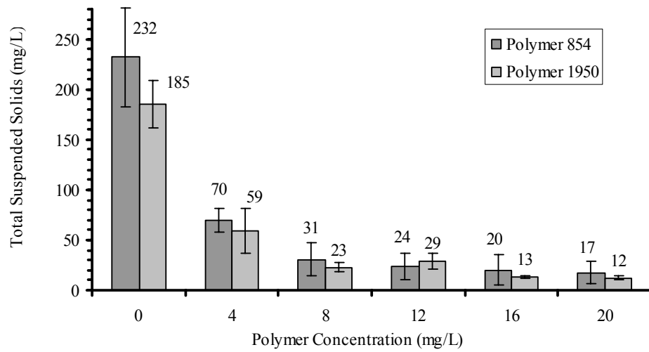
Figure 6. Total Suspended Solids removed using high degree of cationic charge, very high molecular weight polymers.
