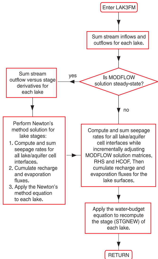
Figure 18. Generalized flow chart of the module LAK3FM.
