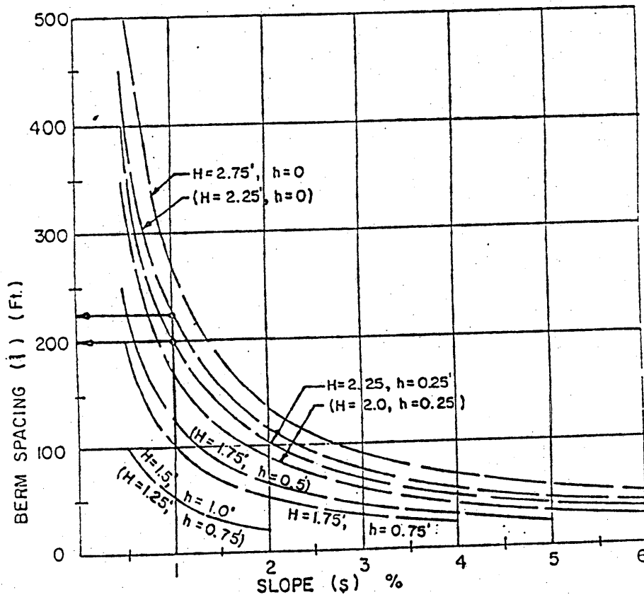
Figure 3 Berm Spacing ( l ) as a Function of Berm Heights ( H, h ) and Slope ( s ) for Swale of Side Slope of 6 on 1
