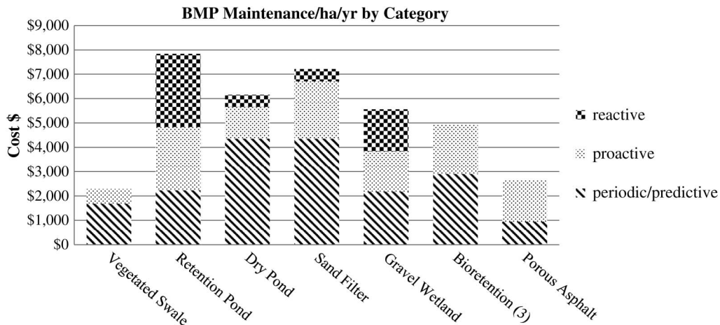
Fig. 2. Annualized maintenance costs per system per hectare of IC treated per maintenance activity classification
